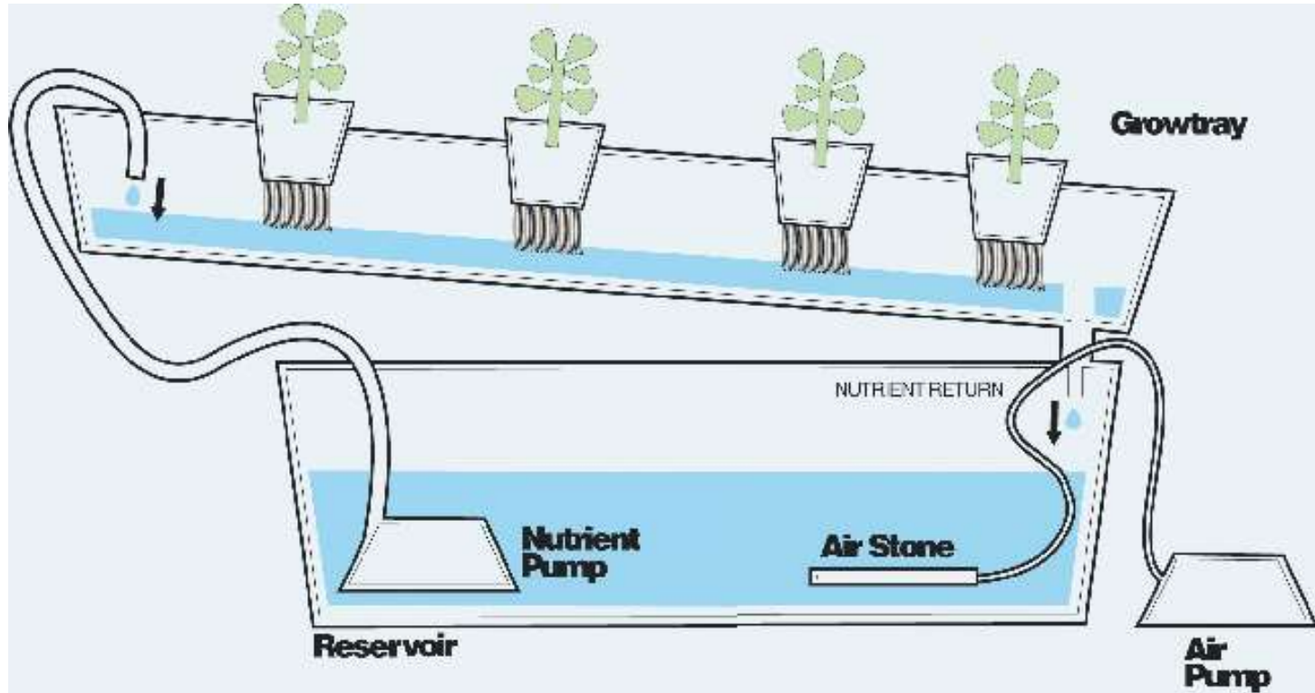
Example of hydroponic installation
